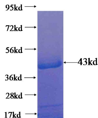
Recombinant human INO80 SDS-PAGE
