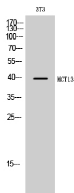
Fig1.; Western Blot analysis of 3T3 cells using MCT13 Polyclonal Antibody
