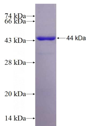
Recombinant Human MAP2K4 SDS-PAGE
