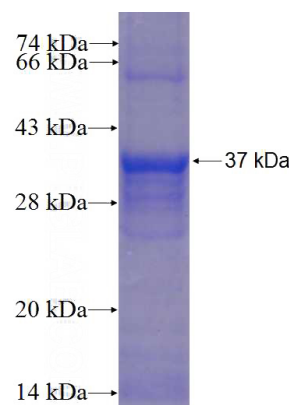
Recombinant Human C17orf58 SDS-PAGE
