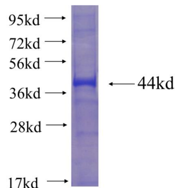
Recombinant human ENTPD4 SDS-PAGE
