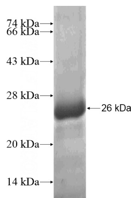
Recombinant Human CAMLG SDS-PAGE
