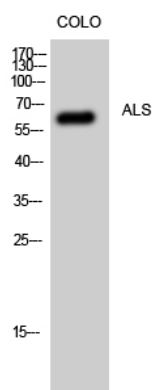
Fig1.; Western Blot analysis of CoLo cells using ALS Polyclonal Antibody
