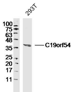
Fig1: Sample: 293T Cell (Human) Lysate at 30 ug; Primary: Anti- C19orf54 at 1/300 dilution; Secondary: IRDye800CW Goat Anti-Rabbit IgG at 1/20000 dilution; Predicted band size: 38kD; Observed band size: 38kD
