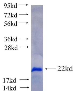
Recombinant human THAP2 SDS-PAGE
