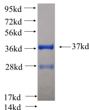
Recombinant human XPO5 SDS-PAGE
