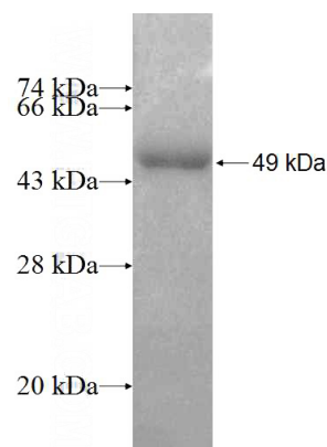
Recombinant Human NSUN4 SDS-PAGE
