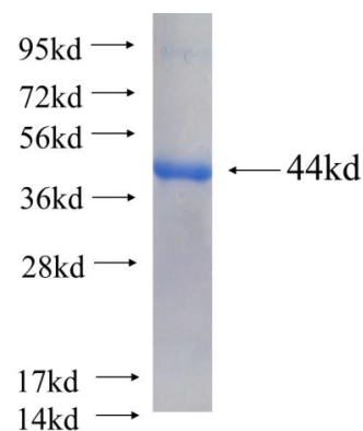
Recombinant human ZNF410 SDS-PAGE
