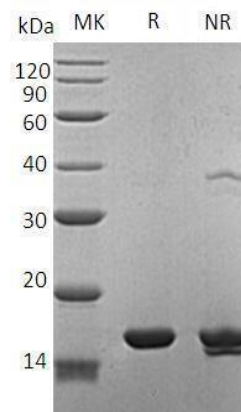
Human FABP7/BLBP/FABPB/MRG (His tag) recombinant protein
