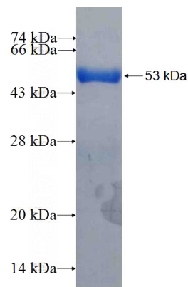
Recombinant Human PEX26 SDS-PAGE
