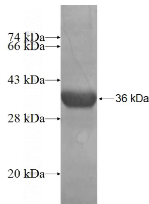
Recombinant Human TEKT1 SDS-PAGE
