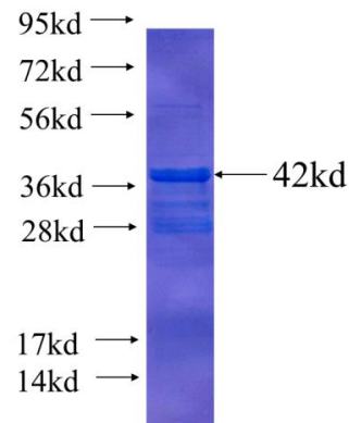
Recombinant human RPL27 SDS-PAGE
