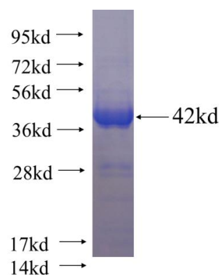
Recombinant human MYBPC3 SDS-PAGE
