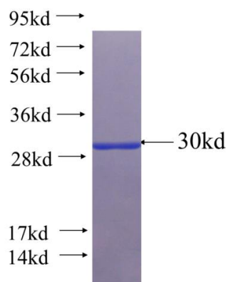
Recombinant Arabidopsis thaliana HIGLE SDS-PAGE
