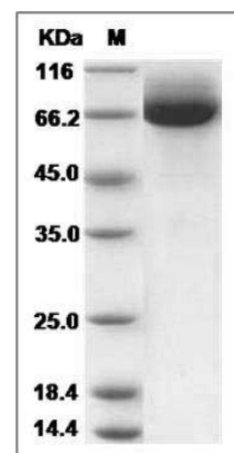
Rat CD36 / SCARB3 Protein (His Tag) SDS-PAGE
