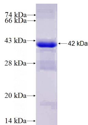
Recombinant Human DUSP12 SDS-PAGE
