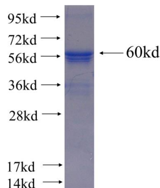
Recombinant human COPE SDS-PAGE
