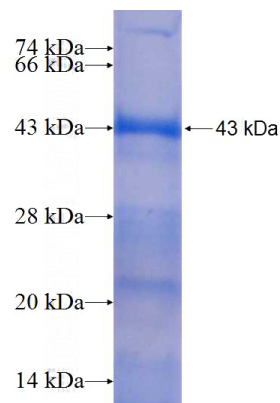
Recombinant Human ARSF SDS-PAGE
