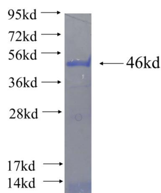
Recombinant human SNW1 SDS-PAGE
