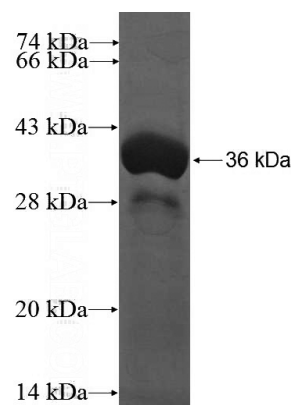
Recombinant Human CDCA8 SDS-PAGE
