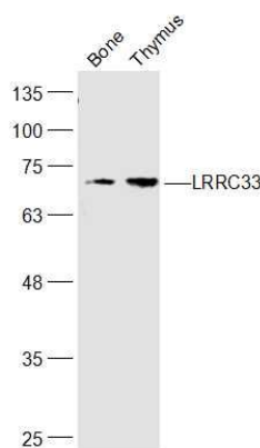
Fig1: Sample:; Bone(Rat) Cell Lysate at 40 ug; Thymus(Rat) Cell Lysate at 40 ug; Primary: Anti-LRRC33 at 1/300 dilution; Secondary: IRDye800CW Goat Anti-Rabbit IgG at 1/20000 dilution; Predicted band size: 74 kD; Observed band size: 74 kD
