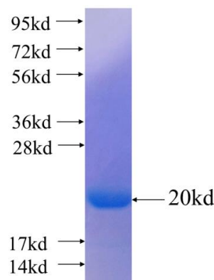
Recombinant human NKX2-2 SDS-PAGE
