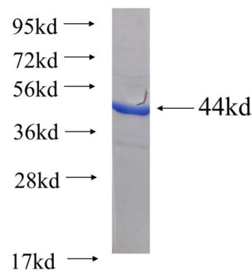
Recombinant human TLR3 SDS-PAGE
