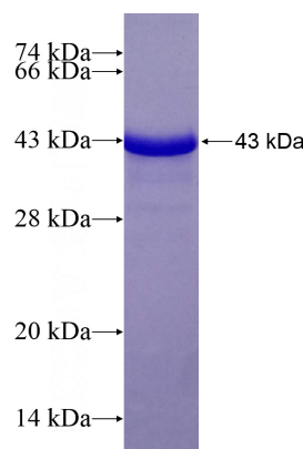
Recombinant Human GAB2 SDS-PAGE
