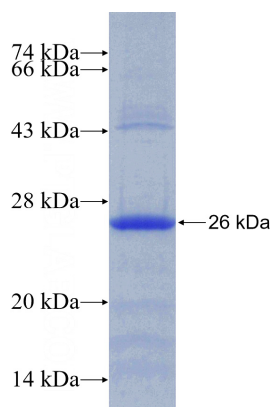
Recombinant Human Caspase 1 SDS-PAGE
