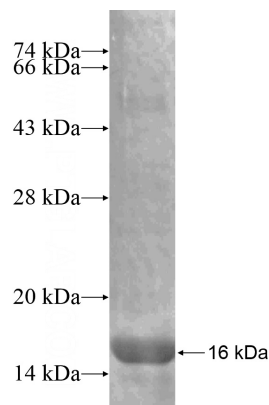
Recombinant Human KRT7 SDS-PAGE
