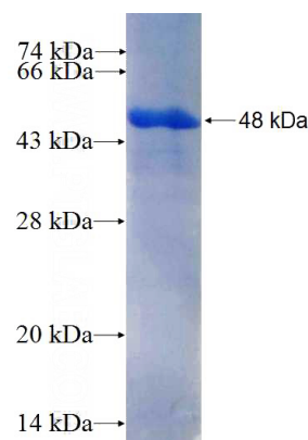
Recombinant Human PPP4R1 SDS-PAGE
