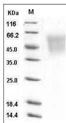
Human CEACAM6 / CD66c Protein (His Tag) SDS-PAGE
