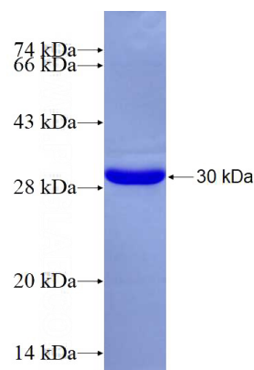
Recombinant Human BZRAP1 SDS-PAGE
