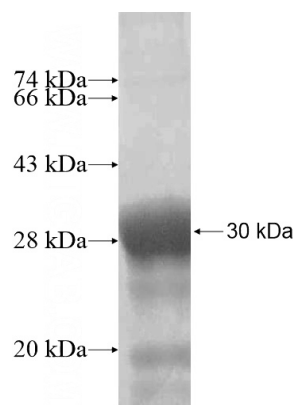
Recombinant Human RNF32 SDS-PAGE
