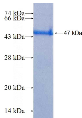
Recombinant Human TIFA SDS-PAGE
