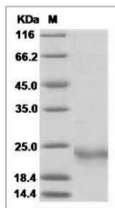
IL19 protein SDS-PAGE
