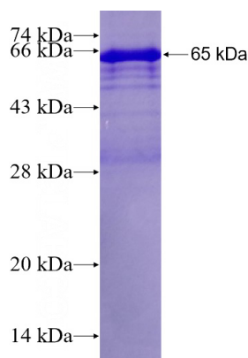
Recombinant Human HDAC2 SDS-PAGE
