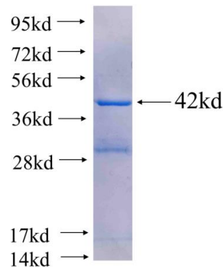
Recombinant human HBE1(Full length) SDS-PAGE
