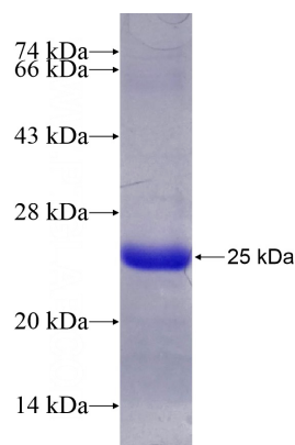
Recombinant Human ARF5 SDS-PAGE
