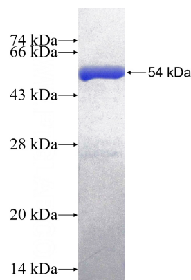
Recombinant Human NANP SDS-PAGE
