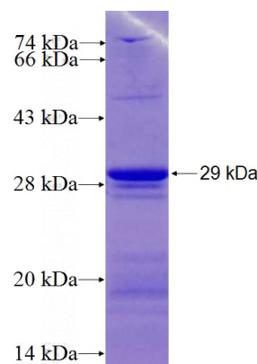
Recombinant Human ATP1B4 SDS-PAGE
