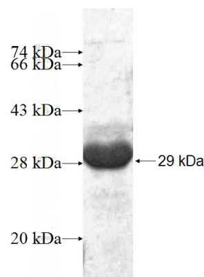
Recombinant Human NUCB1 SDS-PAGE
