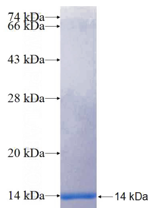
Recombinant Human SGCA SDS-PAGE
