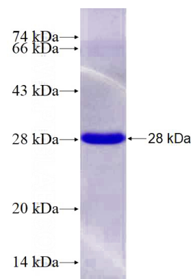
Recombinant Human C11orf35 SDS-PAGE
