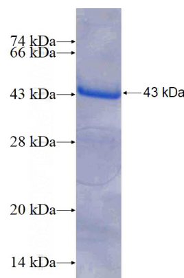
Recombinant Human NSUN5 SDS-PAGE
