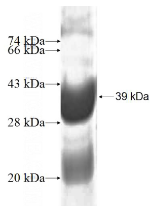
Recombinant Human NDUFA5 SDS-PAGE
