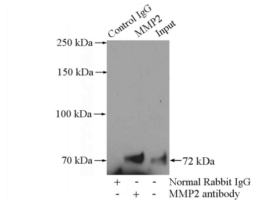
IP Result of anti-MMP2 (IP:Catalog No:112700, 4ug; Detection:Catalog No:112700 1:300) with NIH/3T3 cells lysate 1200ug.
