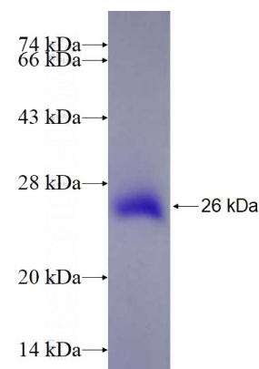
Recombinant Human RNF219 SDS-PAGE
