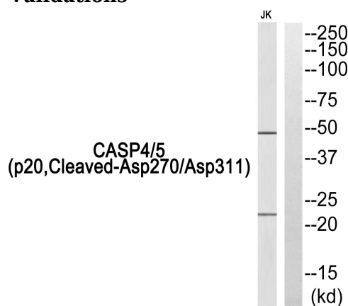
Fig1:; Western blot analysis of Caspase 4/5 (p20, Cleaved-Asp270/Asp311) Antibody. The lane on the right is blocked with the Caspase 4/5 (p20, Cleaved-Asp270/Asp311) peptide.
