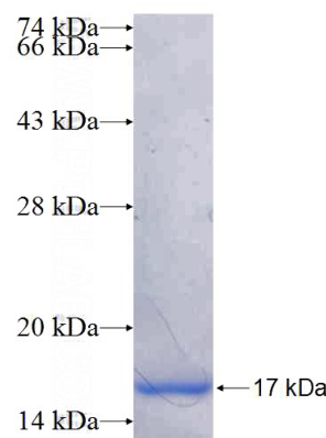
Recombinant Human FLVCR1 SDS-PAGE
